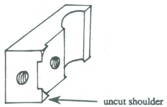
FIG. 11: PIVOT FEATURE MODIFICATION OF THE MODIFIED SQUARE CLAMP DESIGN
