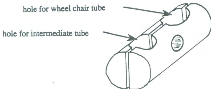
FIG. 3: CLAMP DESIGN FOR THE MARK I PHASE OF THE MAS PROJECT
