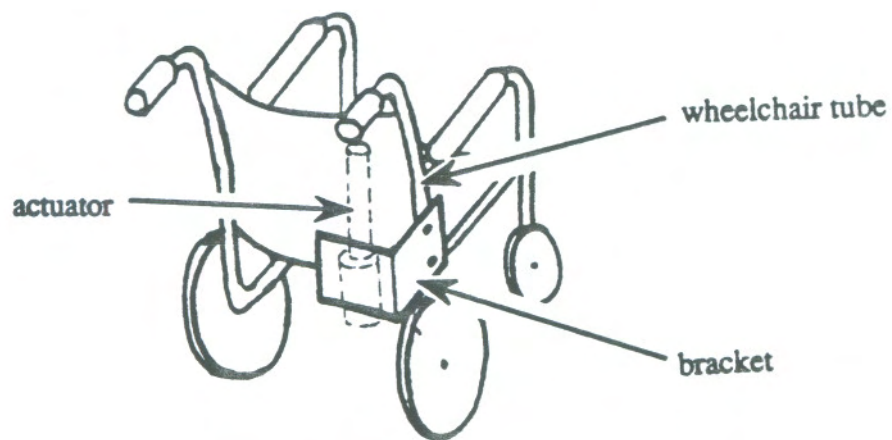
FIG. 2: GENERAL LAYOUT OF THE ATTACHMENT
