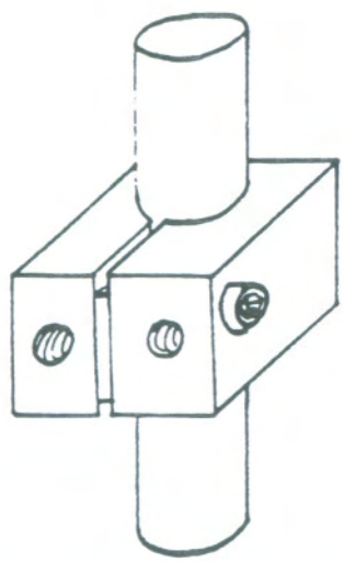
FIG. 10: MODIFIED SQUARE CLAMP DESIGN
