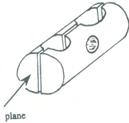
FIG. 4: PLANE FOR ATTACHING THE BRACKET IN MARK I CLAMP DESIGN
