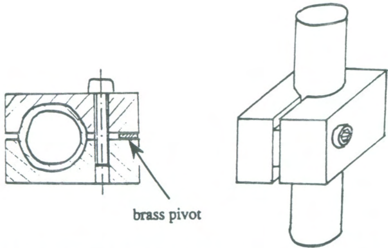
FIG. 9: THE SQUARE CLAMP DESIGN ACCIDENTALLY NOTICED BY THE DESIGNER
