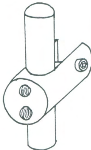
FIG. 8: CLAMP DESIGN WITH CONTINUOUS SLOT
