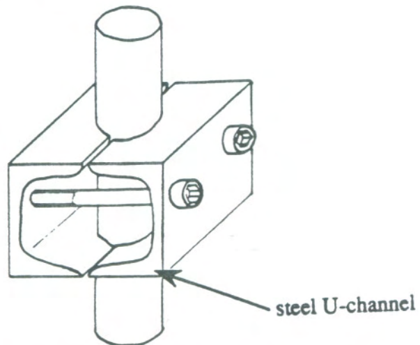
FIG. 15: FINAL CLAMP DESIGN WITH TWO U-CHANNELS
