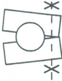
FIG. 6: ATTACHMENT PROBLEM WITH THE MODIFIED MAS I CLAMP DESIGN
