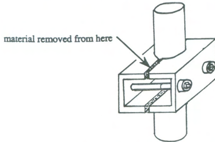
FIG. 14: CLAMP SOLUTION WITH A HOLLOW SQUARE TUBE
