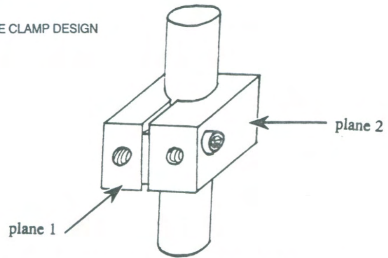
FIG. 12: ALTERNATIVE ATTACHING PLANES IN THE MODIFIED SQUARE CLAMP DESIGN
